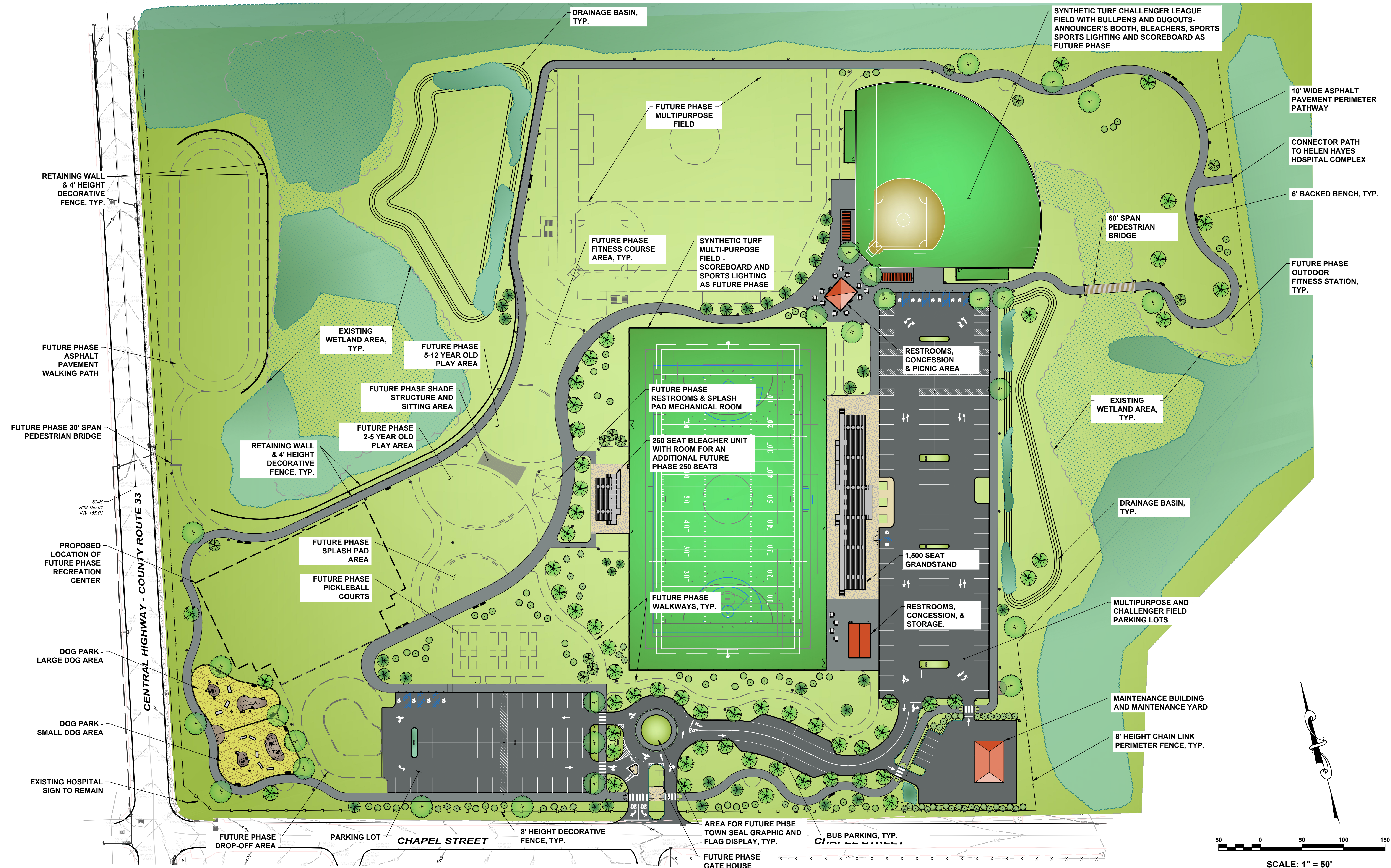
TOWN OF HAVERSTRAW RECREATION COMPLEX ROCKLAND COUNTY, NEW YORK PHASE 1 SITE PLAN - NO ALTERNATES
